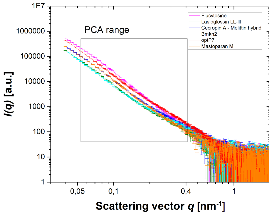
Supplementary Figure 1: SAXS curves with error bars. Each sample was measured 20 times to obtain the SAXS curve. Errors are standard deviations; this error were propagated to the PCA values. For better visualization the errors have been removed from the main Figure 1.
