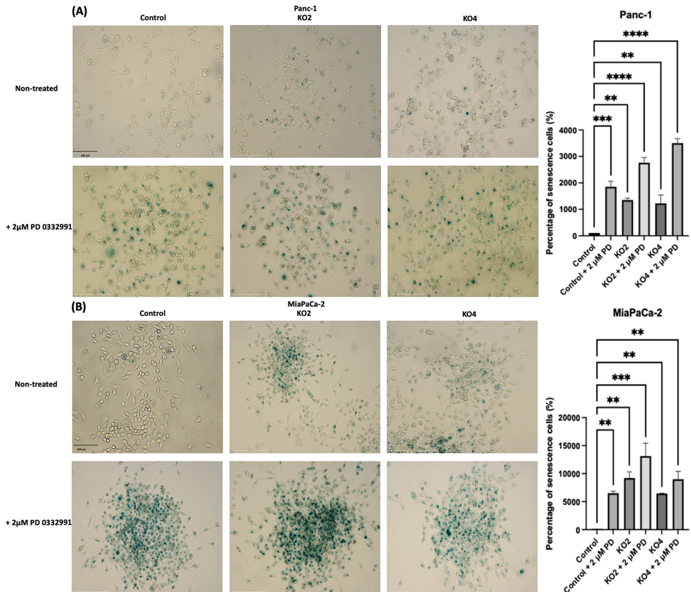
Fig. 5. PD-0332991 treatment triggered cellular senescence in both Panc-1 (A) and MiaPaCa-2 (B) wt cells and their miR-21 KO. Panc-1 and MiaPaCa-2 wt cells and their miR-21 KO were exposed to Senescence \beta -Galactosidase Staining following treatment with the CDK4/6 inhibitor PD-0332991 (2 \mu M, for 24 hrs). After a night of Senescence \beta -Galactosidase staining, cells were examined under a light microscope. The scale bar is 200 \mu m. Graphs show the cell numbers quantification normalised to the control. The histograms represented the mean \pm SD of three technical repeats; data evaluated by One-way ANOVA and Bonferroni's multiple comparison test. Panc-1 and MiaPaCa-2 cells were exposed to PD-0332991 (2 \mu M, for 24 hrs). Exact p-values are indicated * p \leq 0.05 ; ** p \leq 0.01 ; *** p \leq 0.001 ; **** p \leq 0.0001 ; error bars indicate SD.
