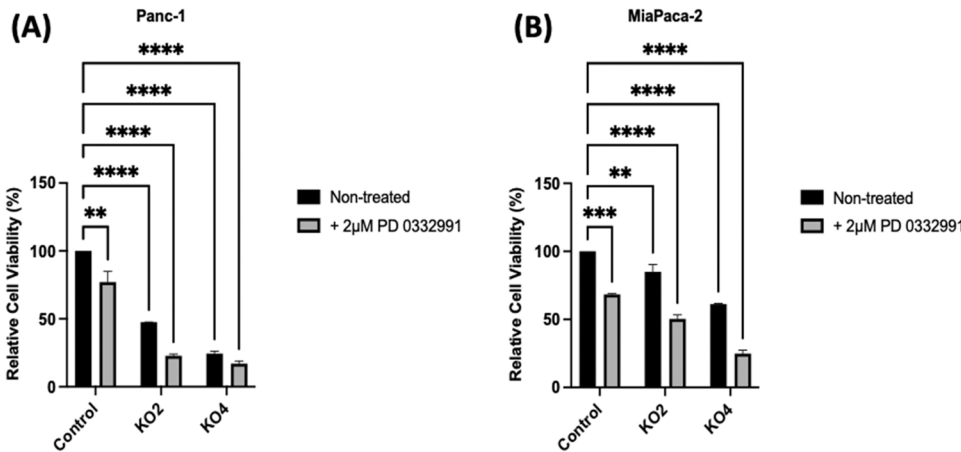
Fig. 2. PD-0332991 decreased cell viability in Panc-1 and MiaPaCa-2 wt cells and their miR-21 KO2. Panc-1 (A) and MiaPaCa-2 (B) were treated with PD-0332991 (2 μM, for 24 hrs). Cells were incubated for 24 hrs and analysed by the MTT method. Cellular viability of treated Panc-1 miR-21 KO2 was also decreased by 50 % compared to non-treated Panc-1 miR-21 KO2 (n = 3; p ≤ 0.01), however mir-21 KO4 did not show the similar trend. Cellular viability of treated MiaPaCa-2 miR-21 KO2 and KO4 was also decreased by 40 % and 59 % compared to non-treated MiaPaCa-2 miR-21 KO2 and KO4 (n = 3; p ≤ 0.0001, for all), respectively. The data are the mean ± SD of three technical repeats evaluated by One-way ANOVA and Bonferroni's multiple comparison test. Exact p-values are indicated * p ≤ 0.05; ** p ≤ 0.01; *** p ≤ 0.001; **** p ≤ 0.0001; error bars indicate SD.
