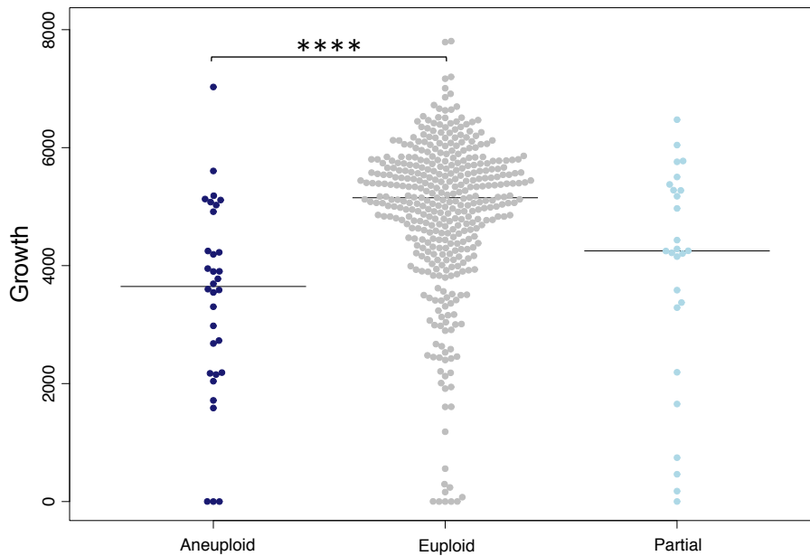
Supplemental Figure 5. Aneuploidy impact on growth for ACTA and Desjardins et al isolates. A) Whole (aneuploid) and partial chromosomal duplications throughout the population. B) Colony size (growth) by ploidy state on YPD at 37°C for both ACTA and Desjardins et al isolates.
