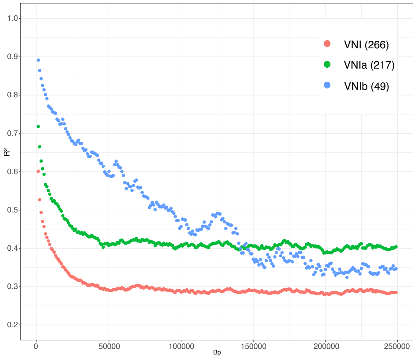
Supplemental Figure 1. Linkage disequilibrium decay over 250kb for lineages VNIa, VNIb, and VNI (VNIa + VNIb). VNI shows 50% LD decay in 30kb.
