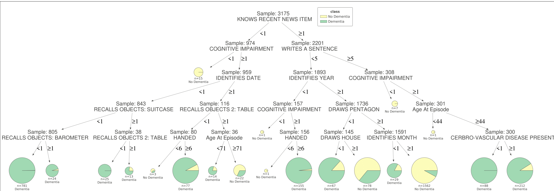
Figure S3: Decision Tree predicts the dementia classes ("Dementia"/"No Dementia") for the Problem (a) using baseline method. The decision trees differ in appearance as well as decision thresholds for certain non-interpretable attributes. The pie charts in leaves show class labels, the proportion of resulting classes and their support size. The branches demonstrate connections between features and their threshold values, leading towards class labels
