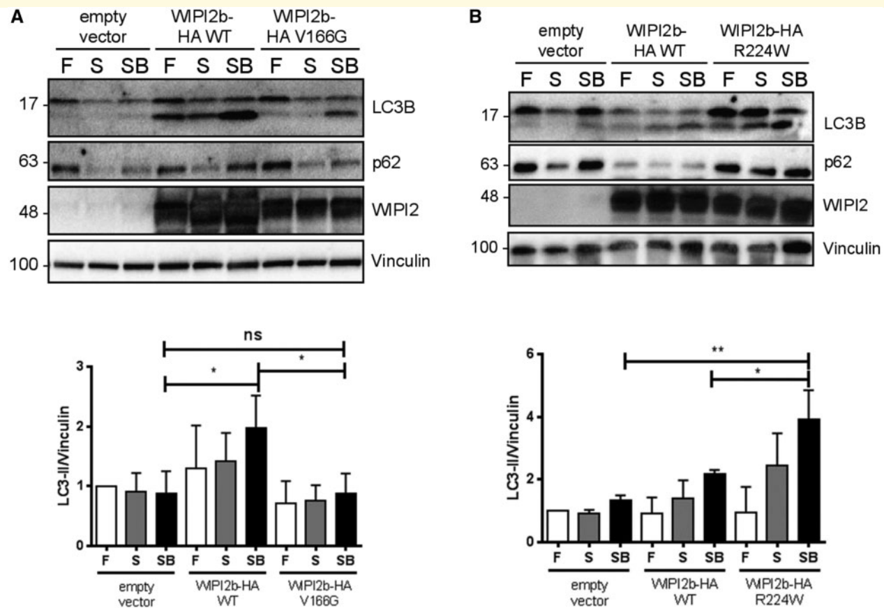
Figure 2 The analysis of autophagic flux upon overexpression of WIPI2b mutants. WIPI2 KO HEK293A cells transiently expressing empty vector, WIPI2b -HA WT or either (A) WIPI2b -HA V166G or (B) WIPI2b -HA R224W, were left untreated or treated with EBSS (amino acid starvation) or EBSS with Bafilomycin A1 for 2 h. The cells were lysed and subjected to SDS-PAGE and Western blot. Antibodies to LC3B, p62, WIPI2 and vinculin were used as indicated. N = 3 , representative experiment is shown. Statistical analysis of LC3-II levels for each blot was performed by one-way ANOVA with Tukey's post-test. SEM from n = 3 . **P < 0.01 . F—fed, untreated; S—EBSS starvation; SB—EBSS starvation + Bafilomycin A1.
