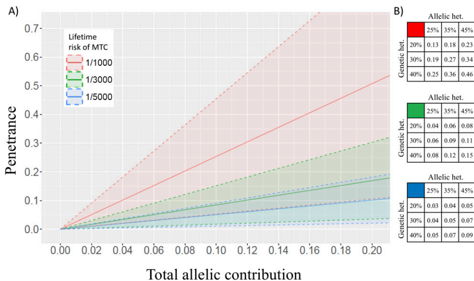
Figure 1. Penetrance for RET p.Val804Met as a function of genetic heterogeneity, allelic heterogeneity, and lifetime risk of MTC. (A) Total allelic contribution (x-axis) is the product of the genetic heterogeneity, multiplied by allelic heterogeneity [e.g., a genetic heterogeneity of 20% and an allelic heterogeneity of 25% gives a total allelic contribution of 5% (or 0.05)]. Penetrance estimates were generated using lifetime risk under three scenarios: a lifetime risk, one in 3000 [a conservative estimate derived from a lifetime risk of MTC in the United States/United Kingdom (green line) and sensitivity testing using lower and higher estimates: one in 5000 (blue line) and one in 1000 (red line)]. Dashed lines and shading indicate 95% confidence intervals (CIs). (B) Point estimates of penetrance are shown by lifetime risk of MTC of one in 3000 (green fill), one in 5000 (blue fill), one in 1000 (red fill) with literature-derived estimates for genetic heterogeneity (25%), and allelic heterogeneity (20%) and sensitivity testing using higher estimates (35% and 45%, 30% and 40%, respectively).
