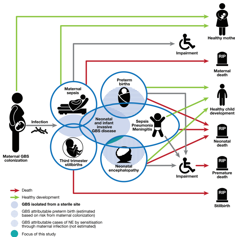
Figure 1. Neonatal encephalopathy (NE) is part of the compartmental model to estimate the burden of group B streptococcal (GBS) disease, as described by Lawn et al [54].
