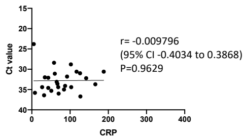
Correlation of lesion orthopox PCR Ct value against CRP
