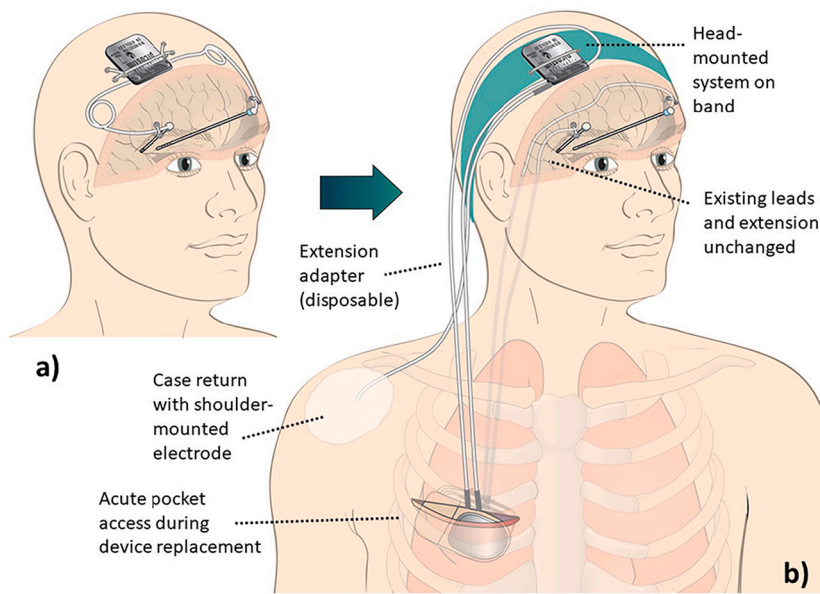
Fig. 5. a) Intended use case for the DyNeuMo Mk-1 for deep brain stimulation. b) Validation experiment set-up. The patient's implanted DBS lead extenders were exposed, at the surgical pocket formed during device changeout. The implanted lead extenders were connected to the externalized DyNeuMo Mk-1 through custom-made disposable DBS lead adapters outside the body. For the duration of acute testing, the commercial replacement IPG was left unconnected. The DyNeuMo was placed over the cranium using a wearable headband to be representative of its intended point of implantation. For the return electrode, a conducting electrode patch was placed on the shoulder and connected to the case. This system configuration allowed for subacute testing during device change-out.
