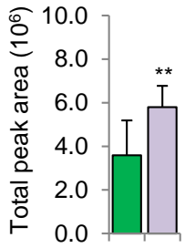
LAMB2_HUMAN ALAEGGSILSR
