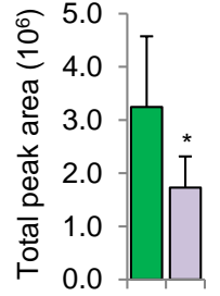
TINAL_HUMAN LDGAWWFLR
