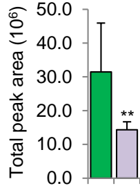
PGS2_HUMAN NLHALILVNNK
