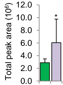
CO1A1_HUMAN GVVGLPGQR
