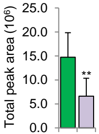
DERM_HUMAN YFESVLR
